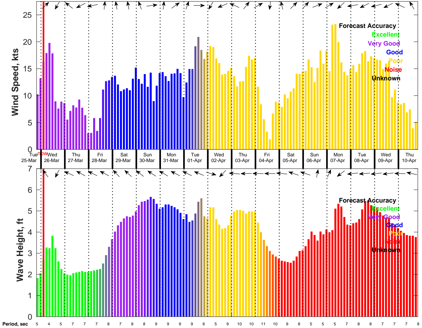
Wind & Wave Forecast for NDBC 41004 from 25-Mar-2025 19:00:00 to 10-Apr-2025 19:00:00
