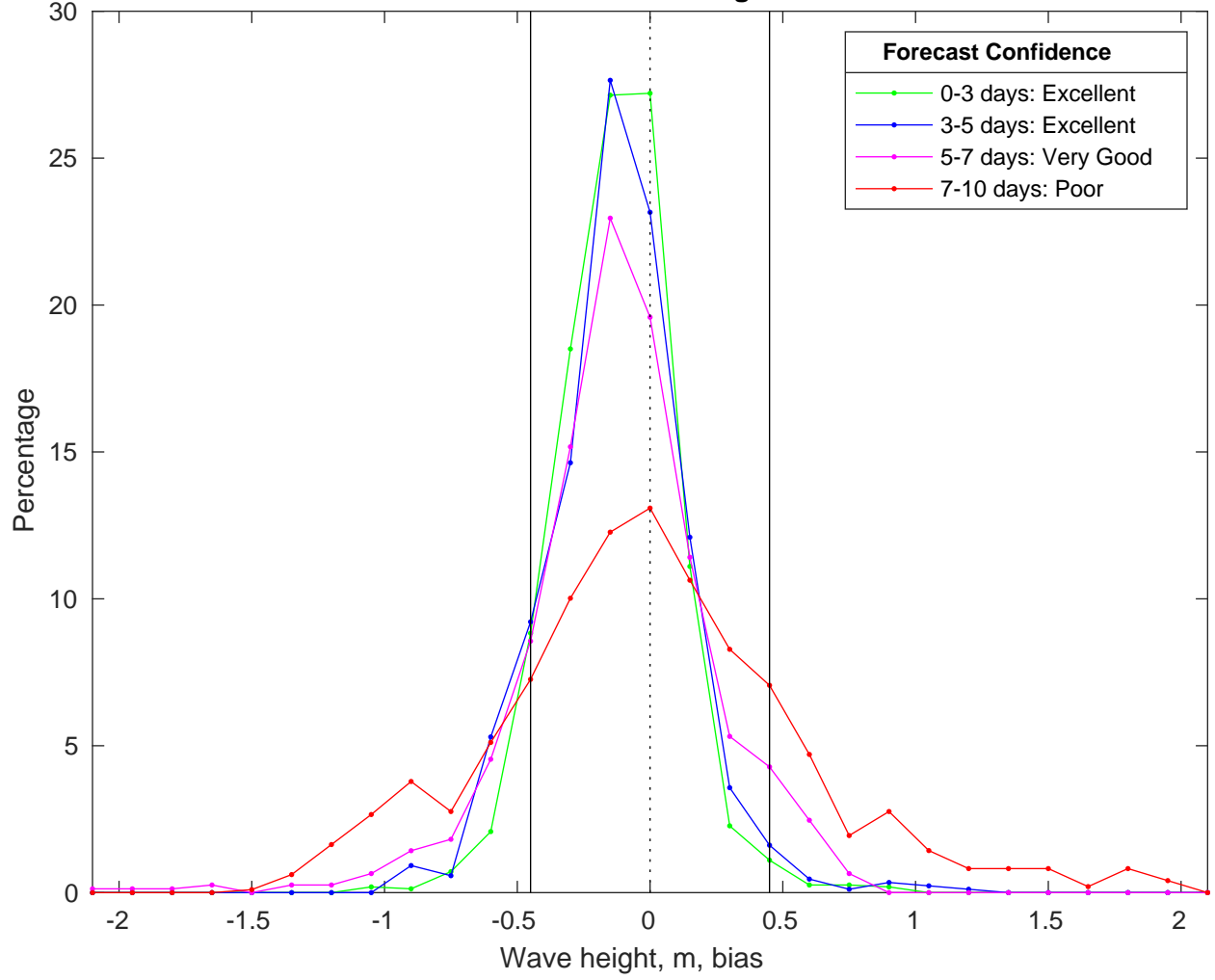
NDBC 41013 vs CMEMS Waves Bias Histogram: 26-Mar-2025
