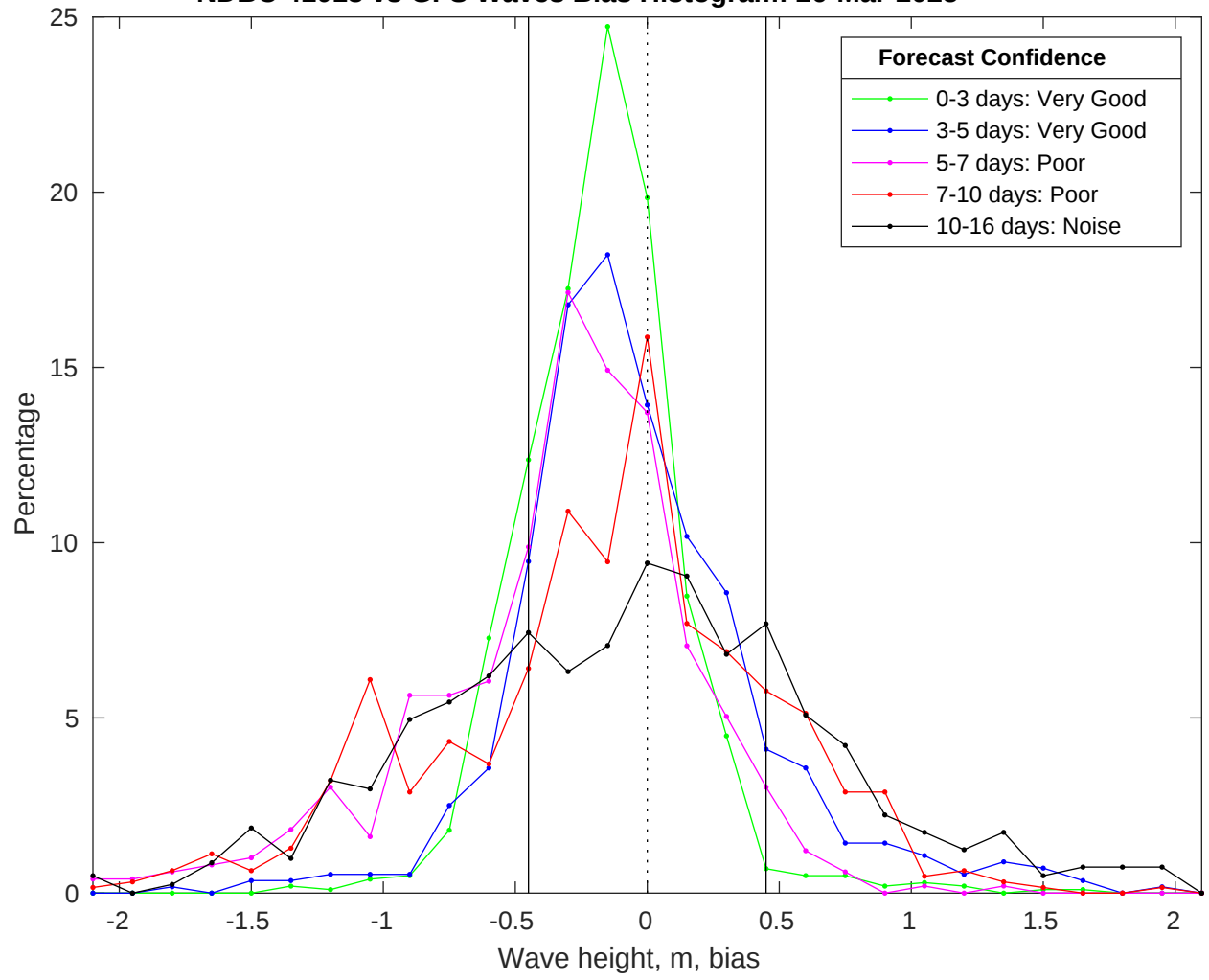
NDBC 41013 vs GFS Waves Bias Histogram: 26-Mar-2025
