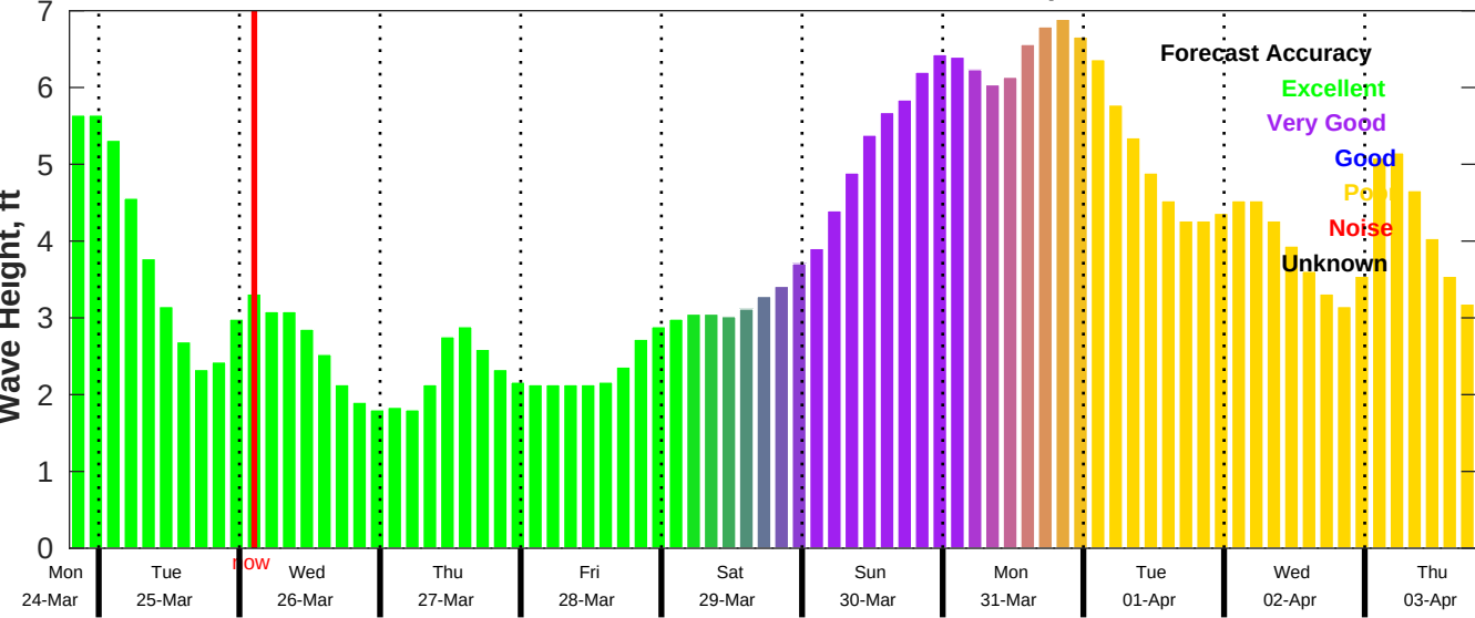
CMEMS Wave Forecast for NDBC 41013 from 24-Mar-2025 19:00:00 to 03-Apr-2025 19:00:00
