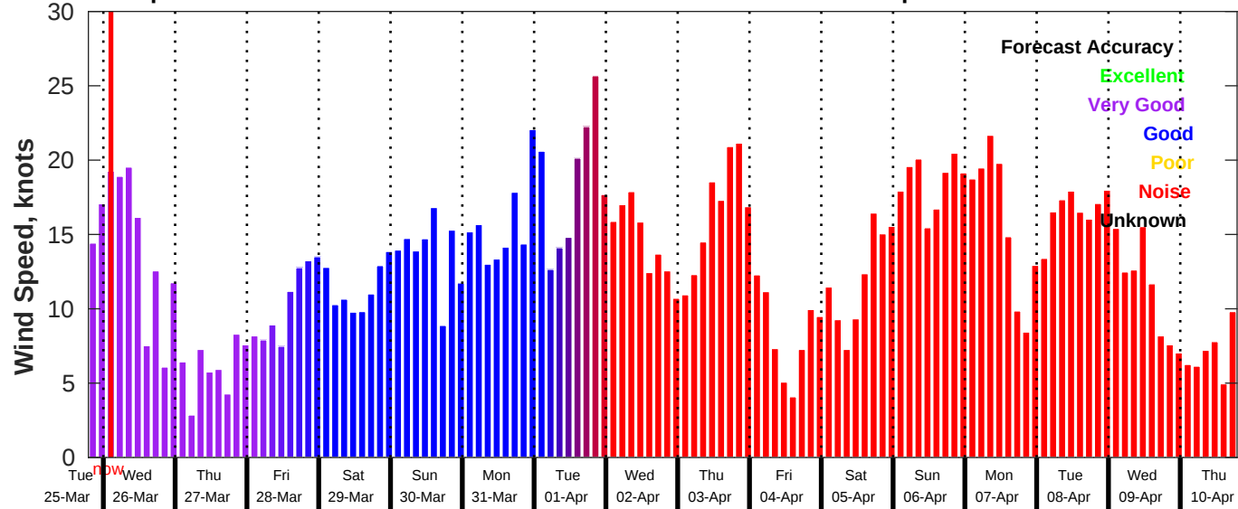
GFS Wind Speed Forecast for NDBC 41013 from 25-Mar-2025 19:00:00 to 10-Apr-2025 19:00:00
