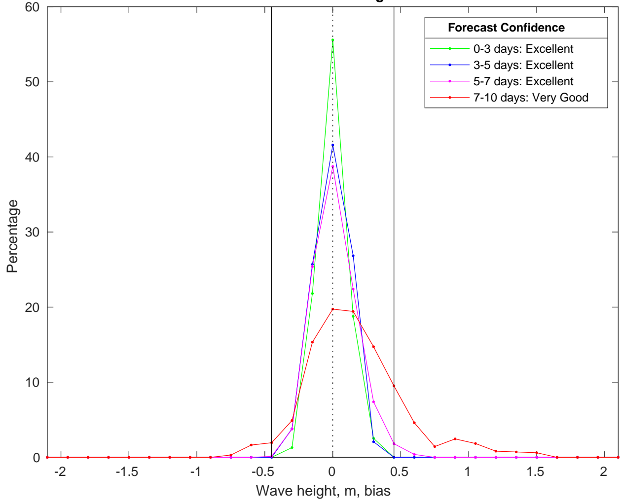
NDBC 41040 vs CMEMS Waves Bias Histogram: 26-Mar-2025
