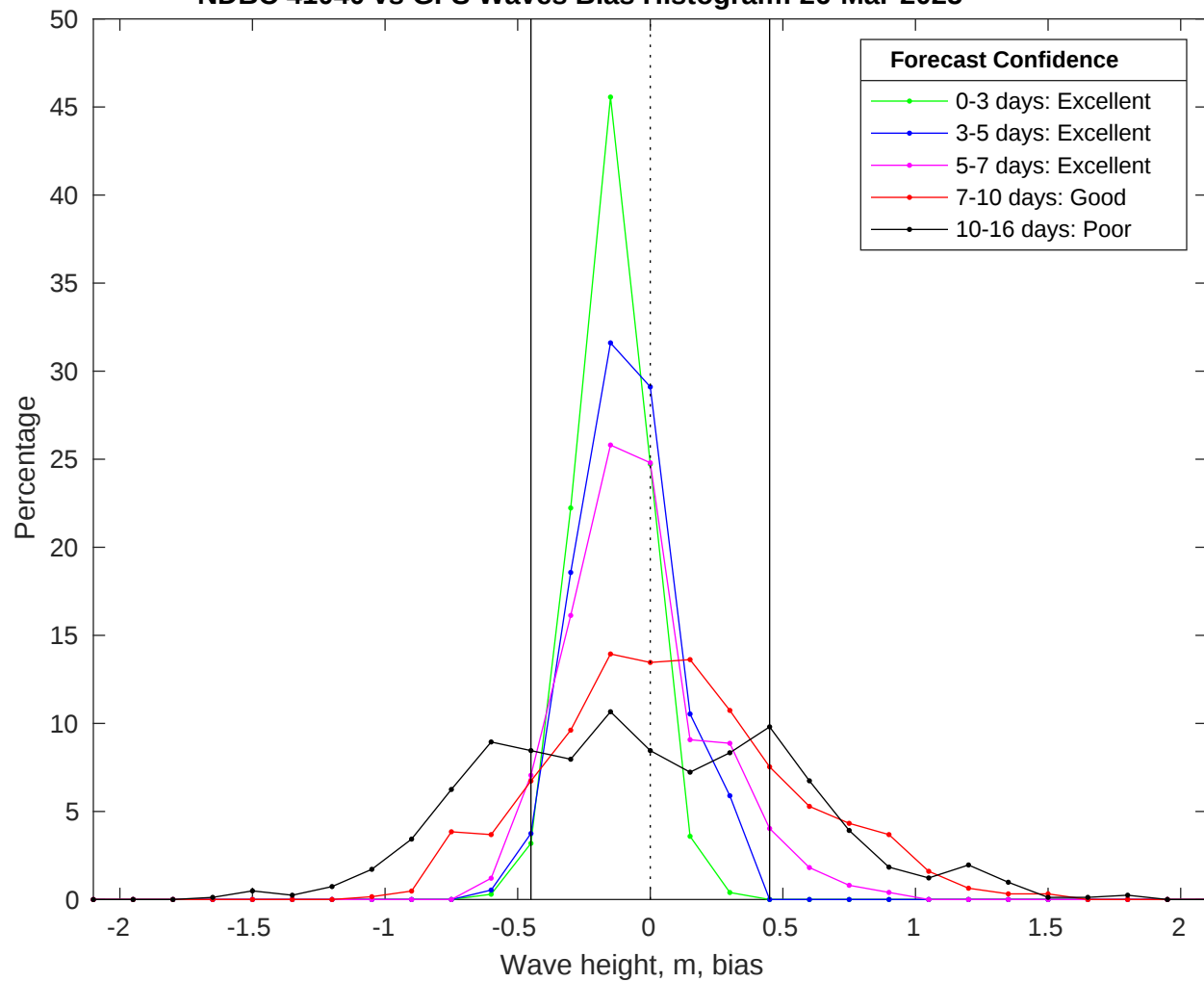
NDBC 41040 vs GFS Waves Bias Histogram: 26-Mar-2025
