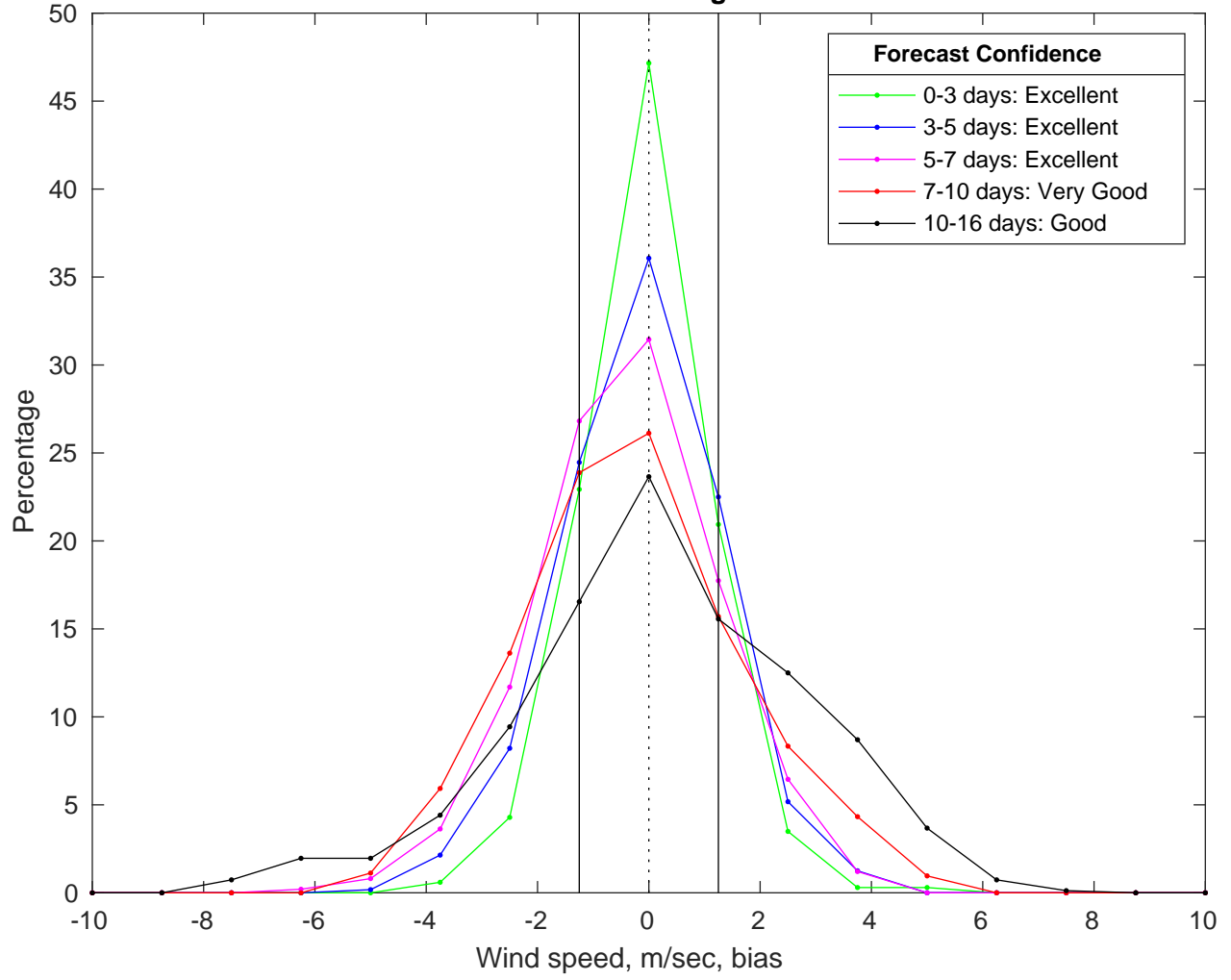
NDBC 41040 vs GFS Winds Bias Histogram: 26-Mar-2025
