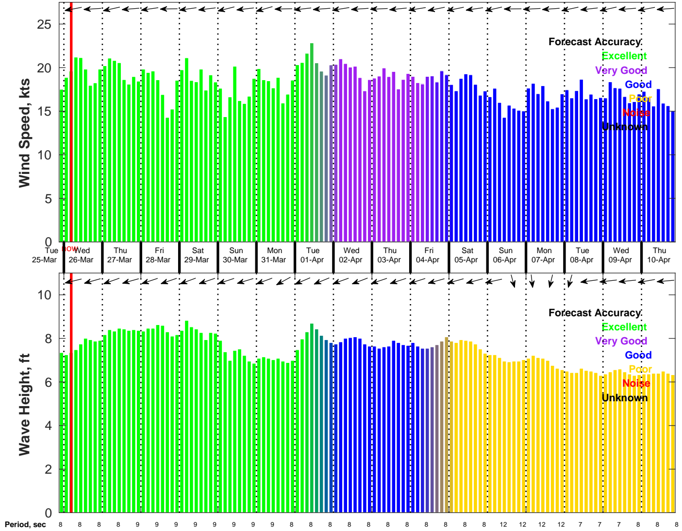
Wind & Wave Forecast for NDBC 41040 from 25-Mar-2025 21:00:00 to 10-Apr-2025 21:00:00
