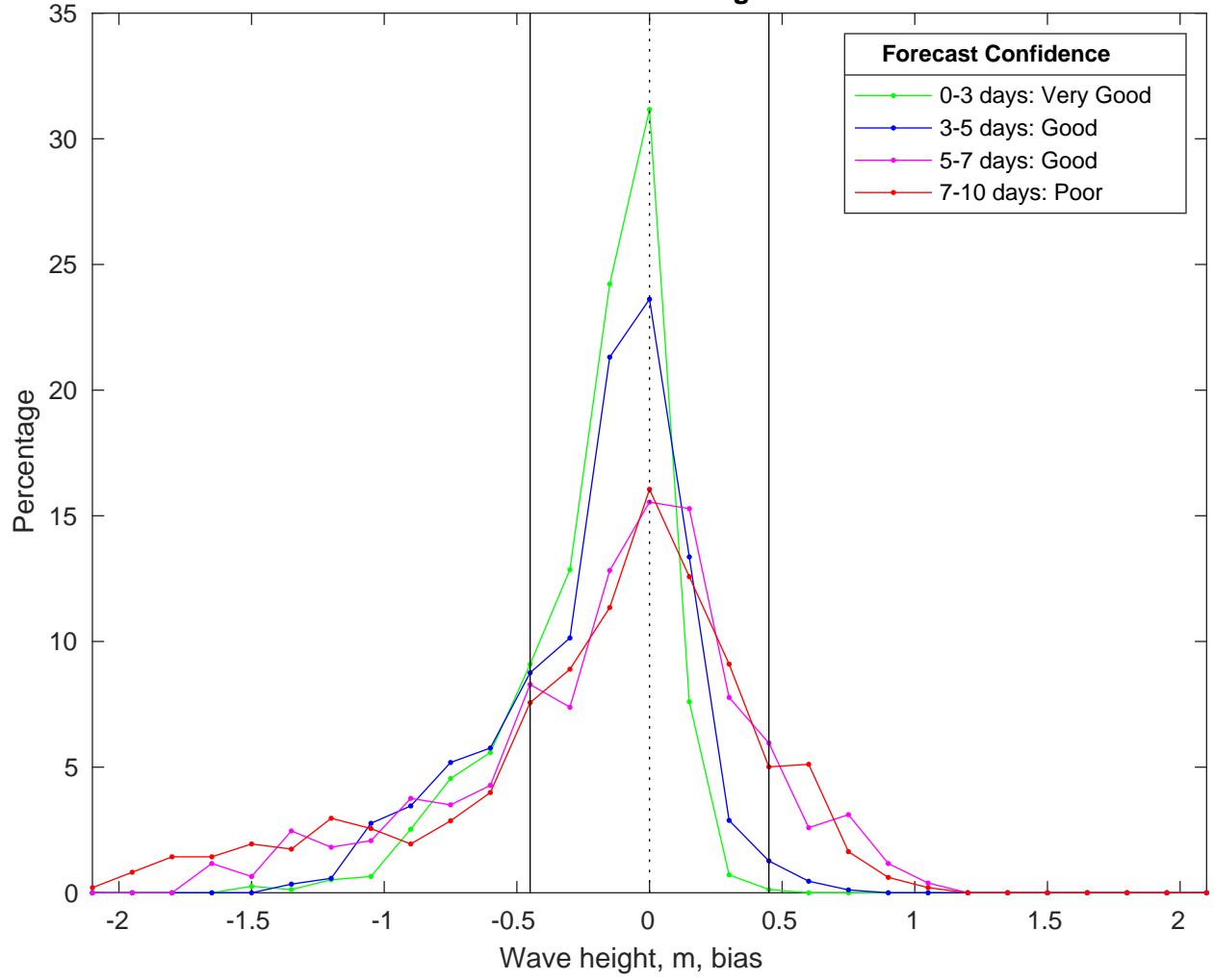
NDBC 42019 vs CMEMS Waves Bias Histogram: 26-Mar-2025
