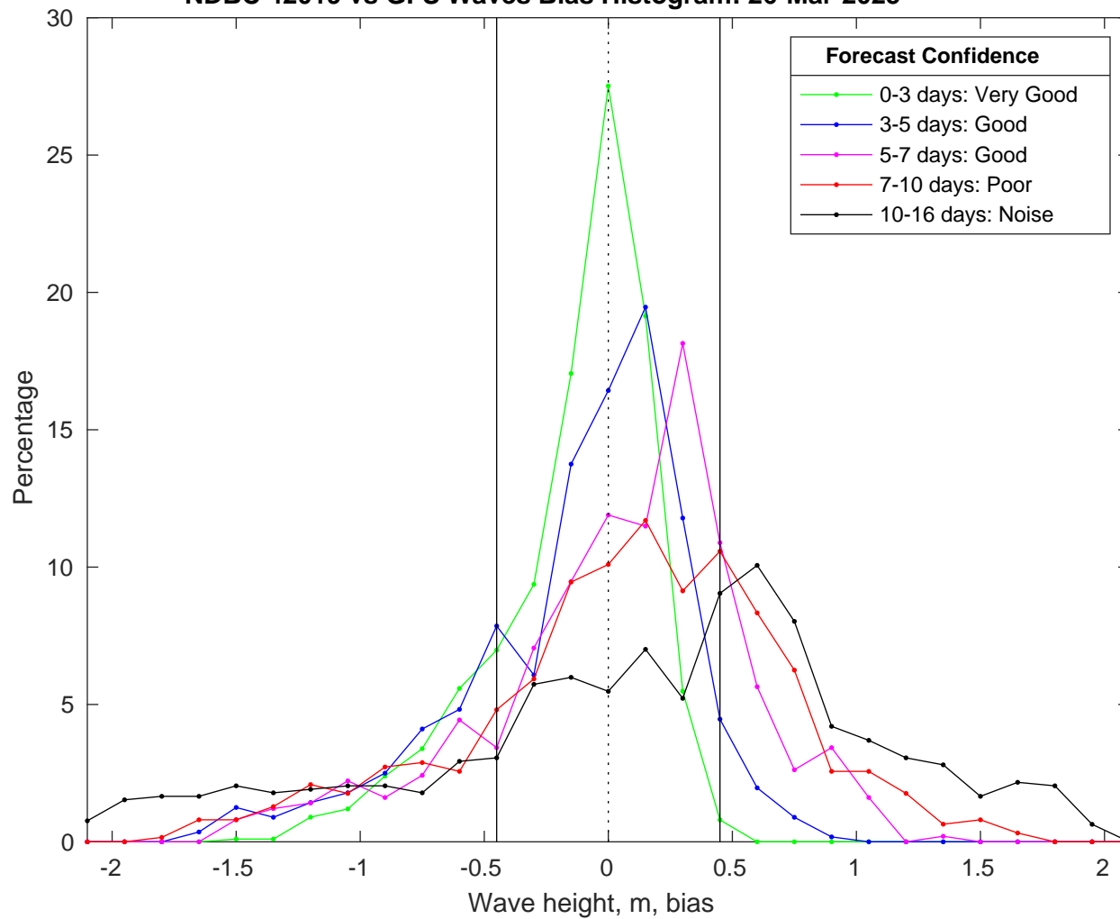
NDBC 42019 vs GFS Waves Bias Histogram: 26-Mar-2025
