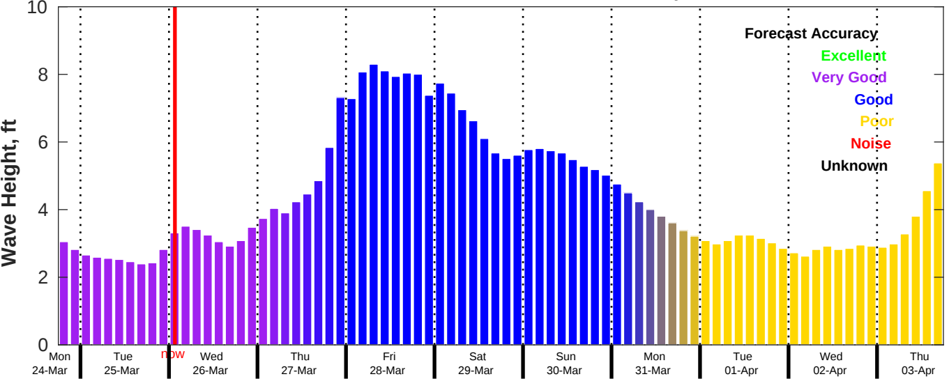
CMEMS Wave Forecast for NDBC 42019 from 24-Mar-2025 18:00:00 to 03-Apr-2025 18:00:00
