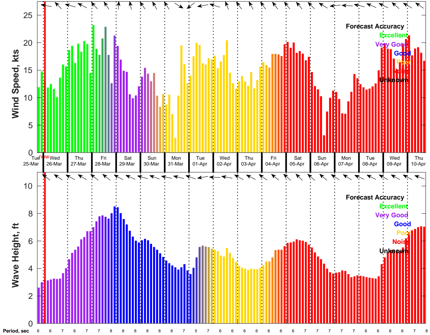
Wind & Wave Forecast for NDBC 42019 from 25-Mar-2025 18:00:00 to 10-Apr-2025 18:00:00
