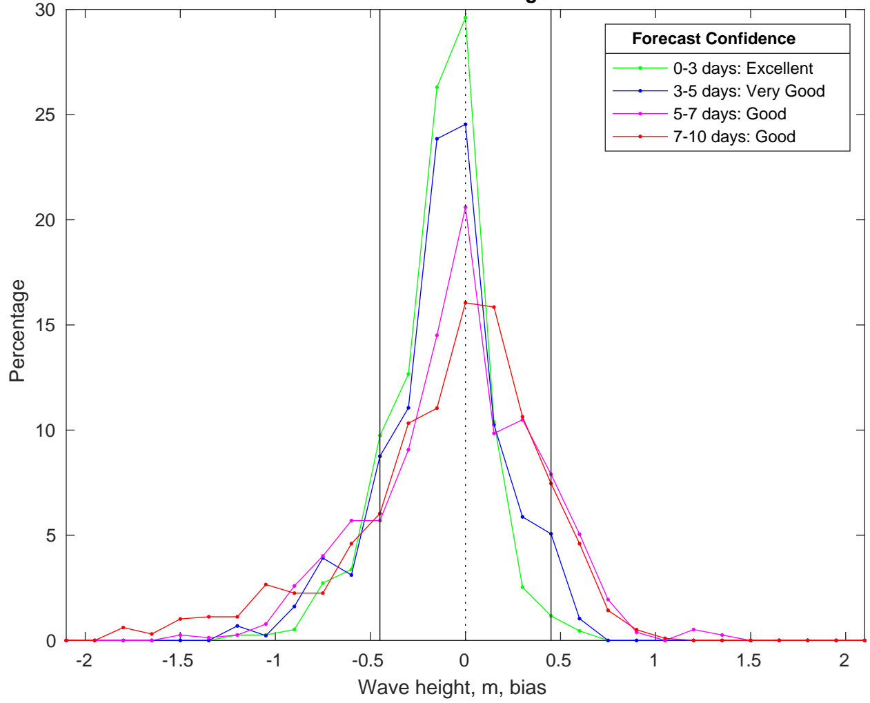
NDBC 42020 vs CMEMS Waves Bias Histogram: 26-Mar-2025
