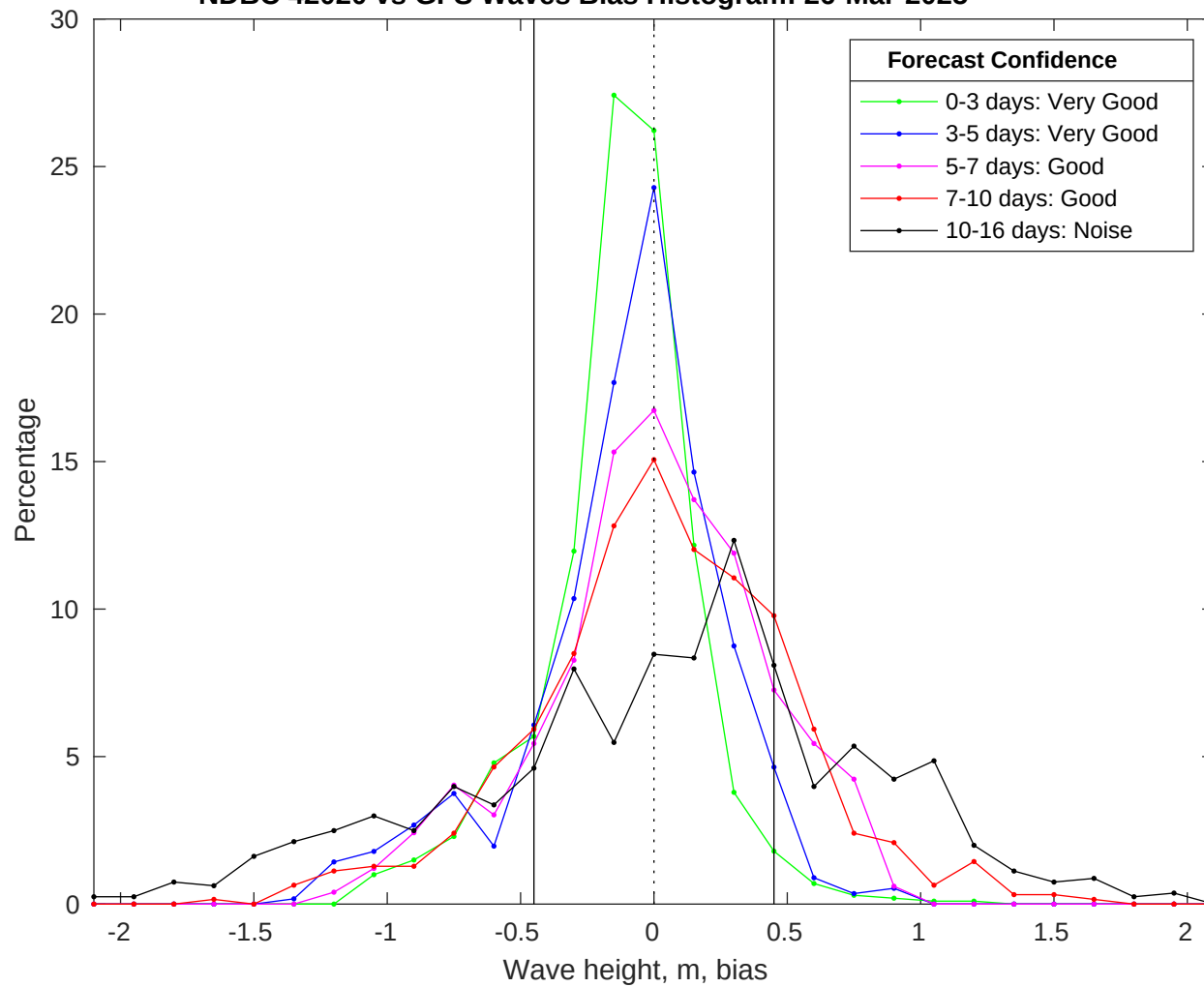
NDBC 42020 vs GFS Waves Bias Histogram: 26-Mar-2025
