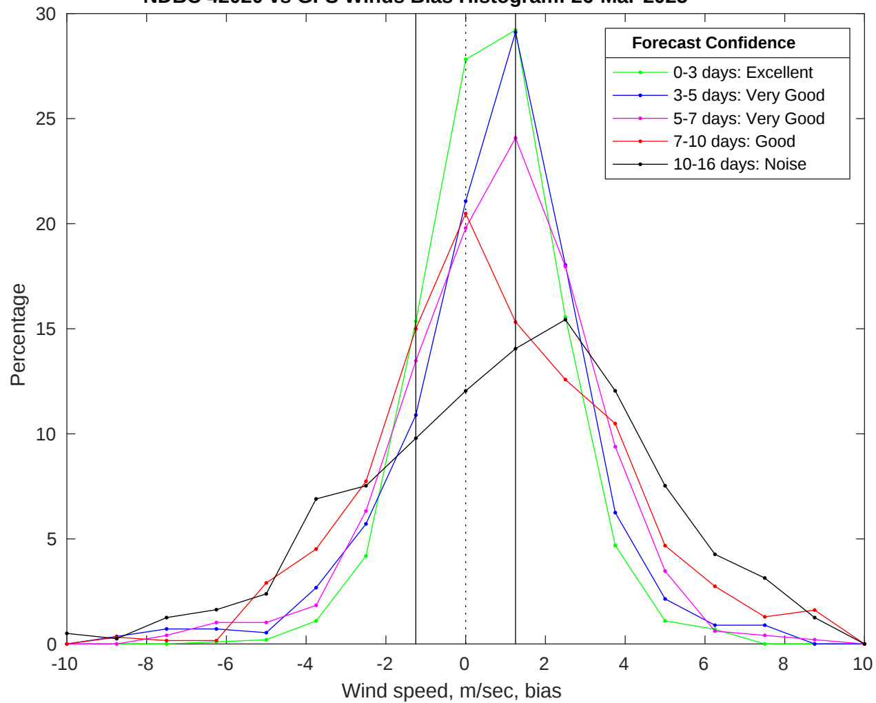
NDBC 42020 vs GFS Winds Bias Histogram: 26-Mar-2025
