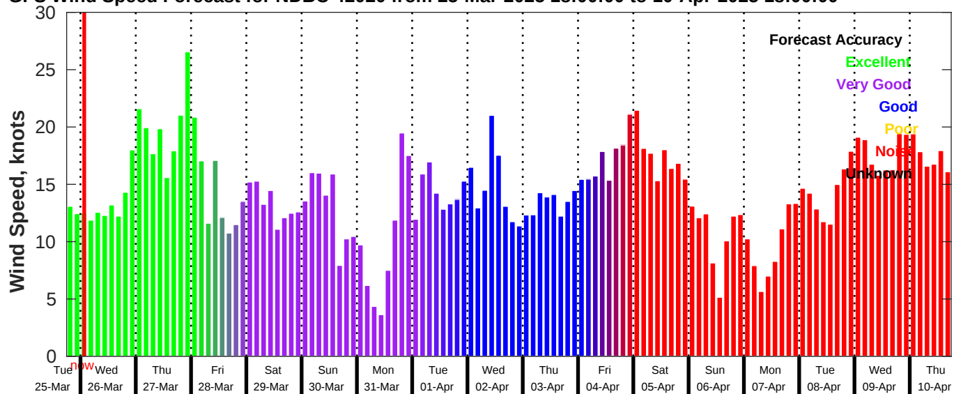
GFS Wind Speed Forecast for NDBC 42020 from 25-Mar-2025 18:00:00 to 10-Apr-2025 18:00:00
