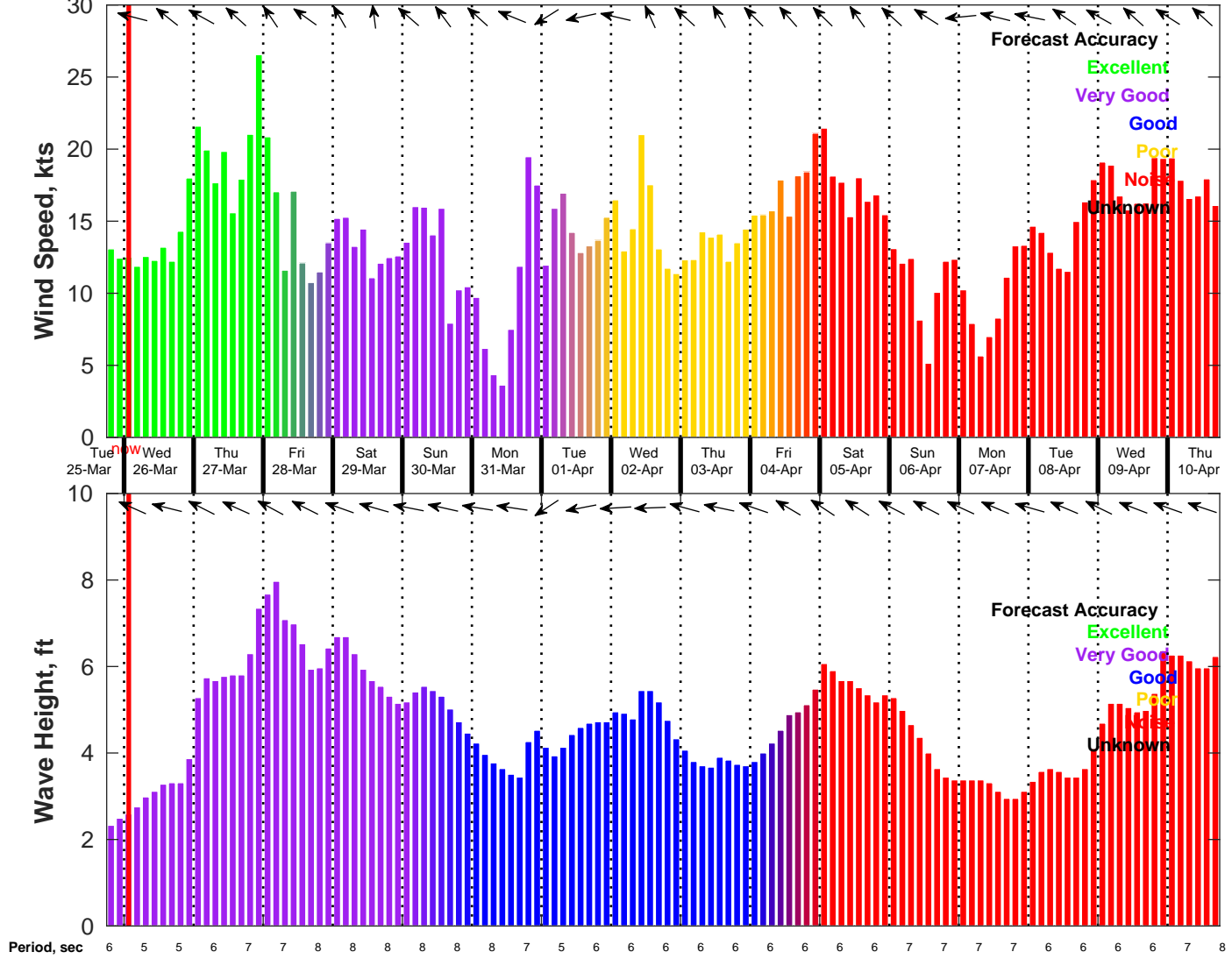
Wind & Wave Forecast for NDBC 42020 from 25-Mar-2025 18:00:00 to 10-Apr-2025 18:00:00
