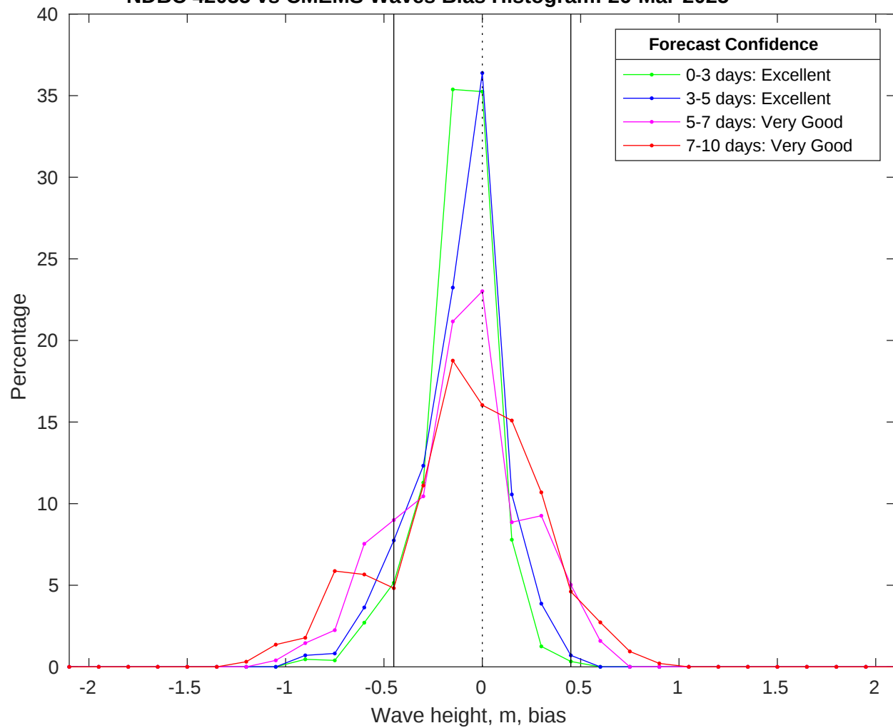
NDBC 42035 vs CMEMS Waves Bias Histogram: 26-Mar-2025
