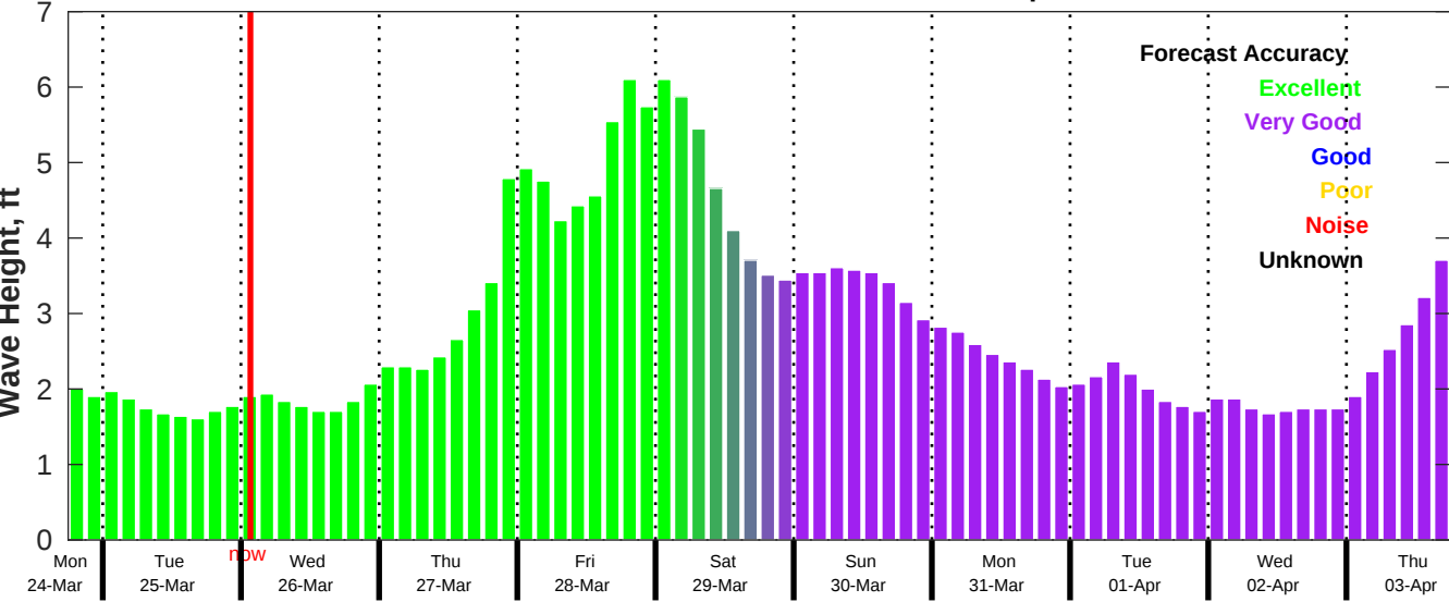
CMEMS Wave Forecast for NDBC 42035 from 24-Mar-2025 18:00:00 to 03-Apr-2025 18:00:00
