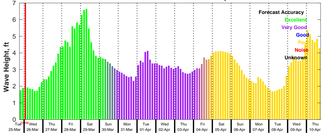
GFS Wave Forecast for NDBC 42035 from 25-Mar-2025 18:00:00 to 10-Apr-2025 18:00:00
