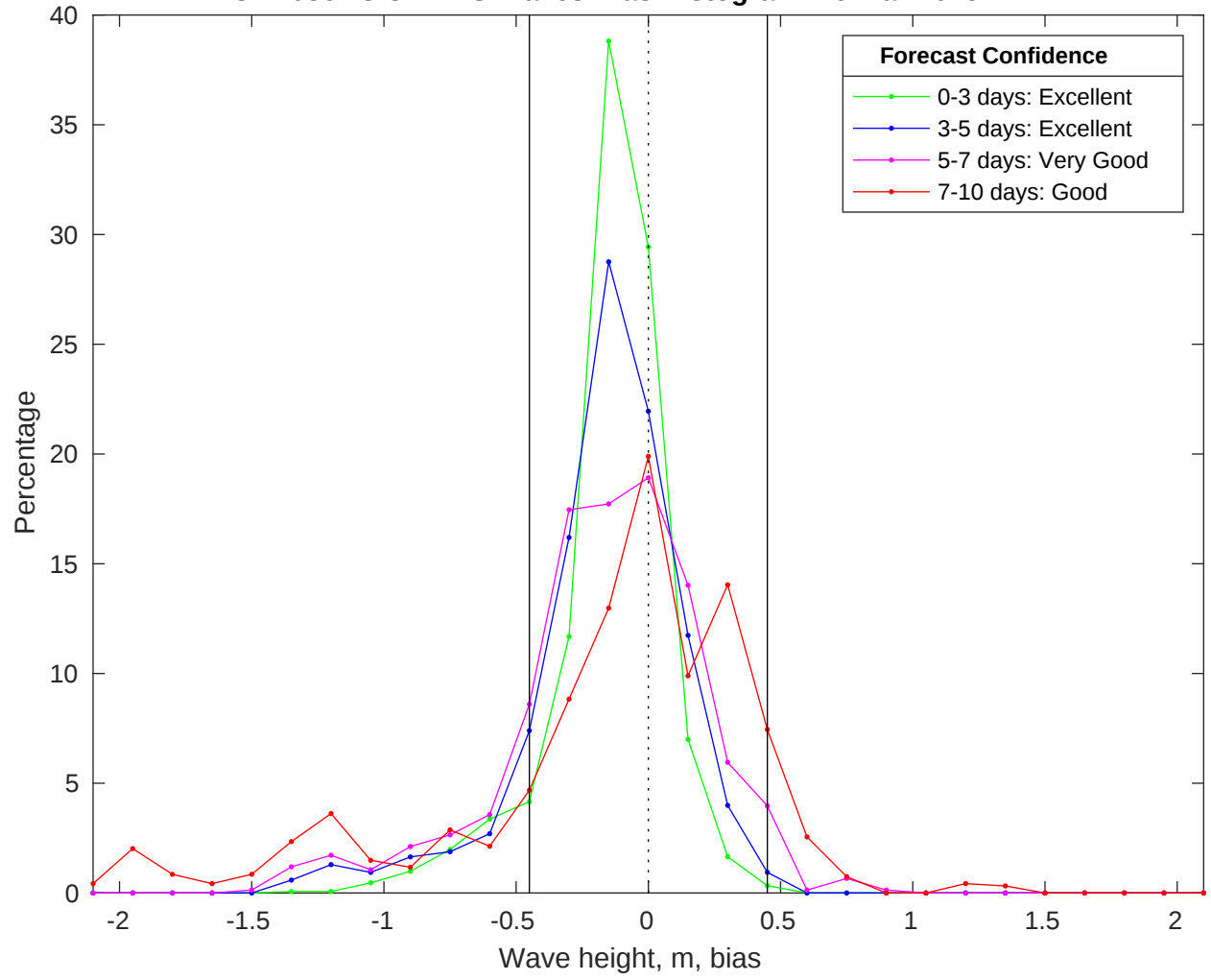
NDBC 42036 vs CMEMS Waves Bias Histogram: 26-Mar-2025
