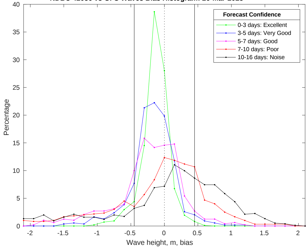
NDBC 42036 vs GFS Waves Bias Histogram: 26-Mar-2025
