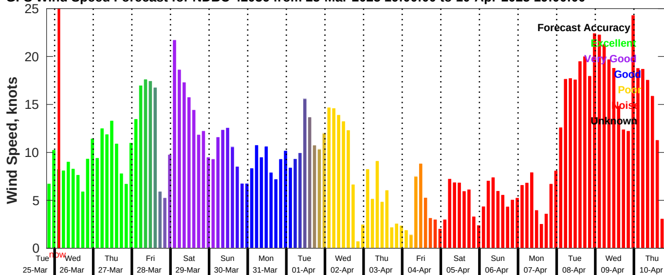
GFS Wind Speed Forecast for NDBC 42036 from 25-Mar-2025 19:00:00 to 10-Apr-2025 19:00:00
