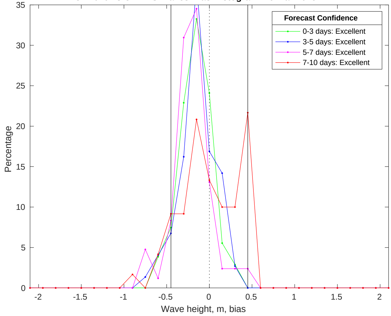
NDBC 42040 vs CMEMS Waves Bias Histogram: 26-Mar-2025
