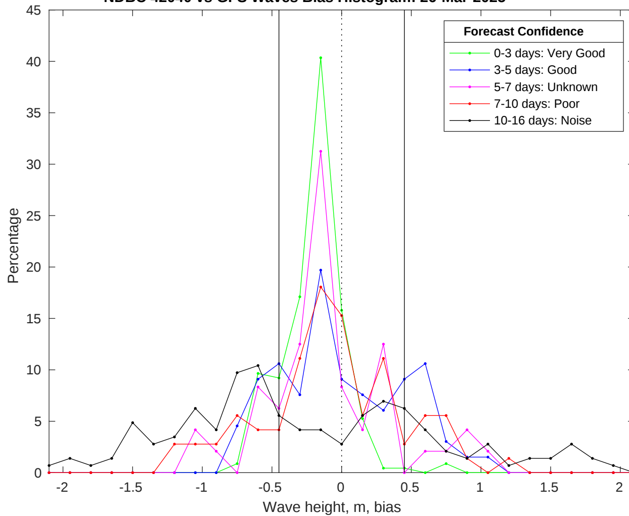
NDBC 42040 vs GFS Waves Bias Histogram: 26-Mar-2025
