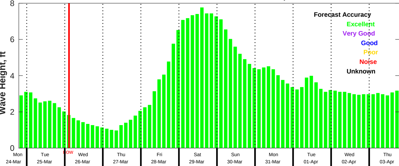
CMEMS Wave Forecast for NDBC 42040 from 24-Mar-2025 19:00:00 to 03-Apr-2025 19:00:00
