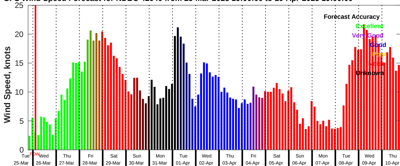
GFS Wind Speed Forecast for NDBC 42040 from 25-Mar-2025 19:00:00 to 10-Apr-2025 19:00:00
