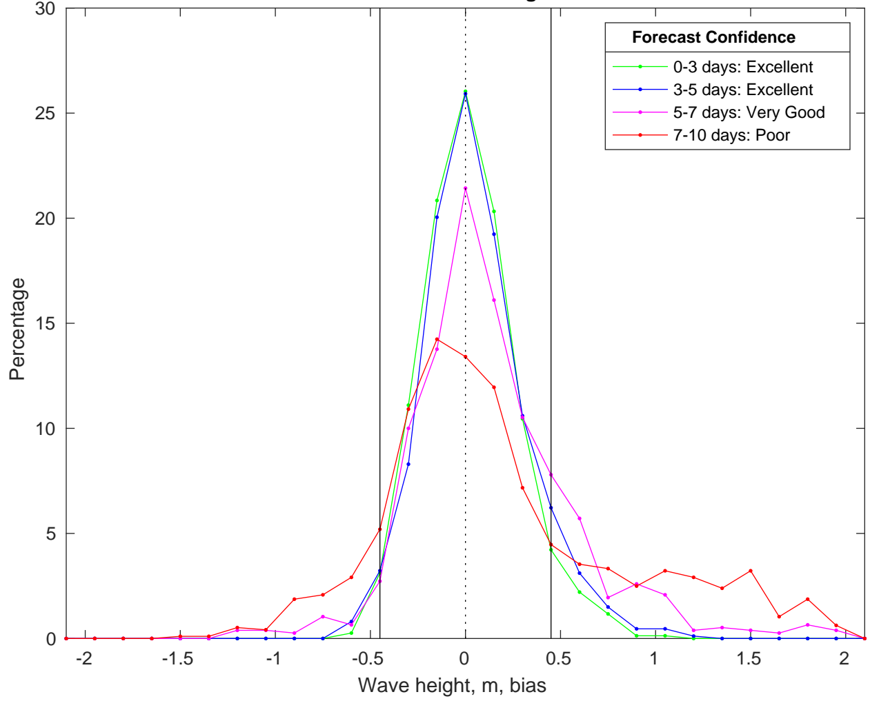
NDBC 46011 vs CMEMS Waves Bias Histogram: 26-Mar-2025
