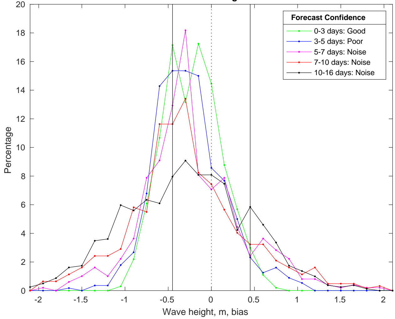
NDBC 46011 vs GFS Waves Bias Histogram: 26-Mar-2025
