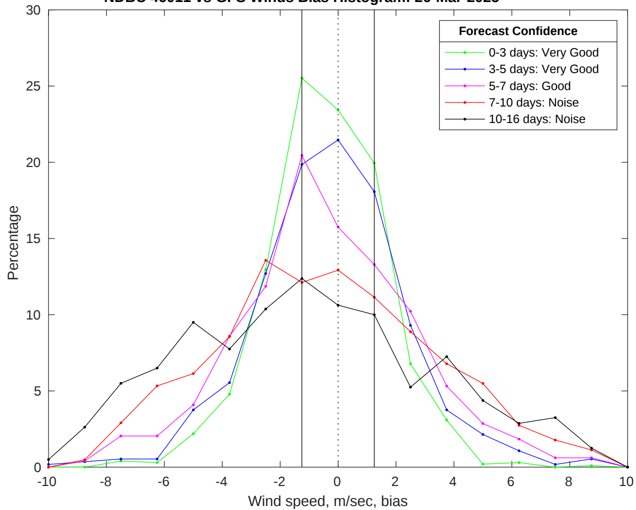
NDBC 46011 vs GFS Winds Bias Histogram: 26-Mar-2025
