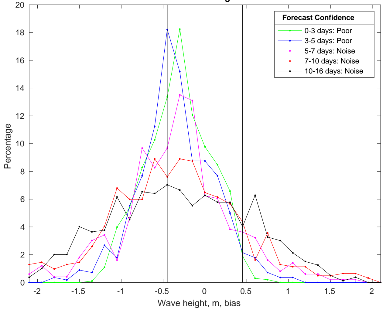
NDBC 46028 vs GFS Waves Bias Histogram: 26-Mar-2025
