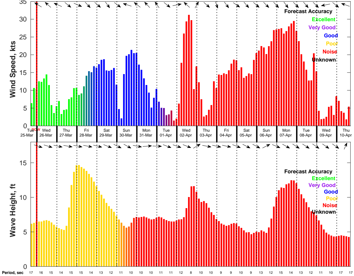
Wind & Wave Forecast for NDBC 46028 from 25-Mar-2025 16:00:00 to 10-Apr-2025 16:00:00
