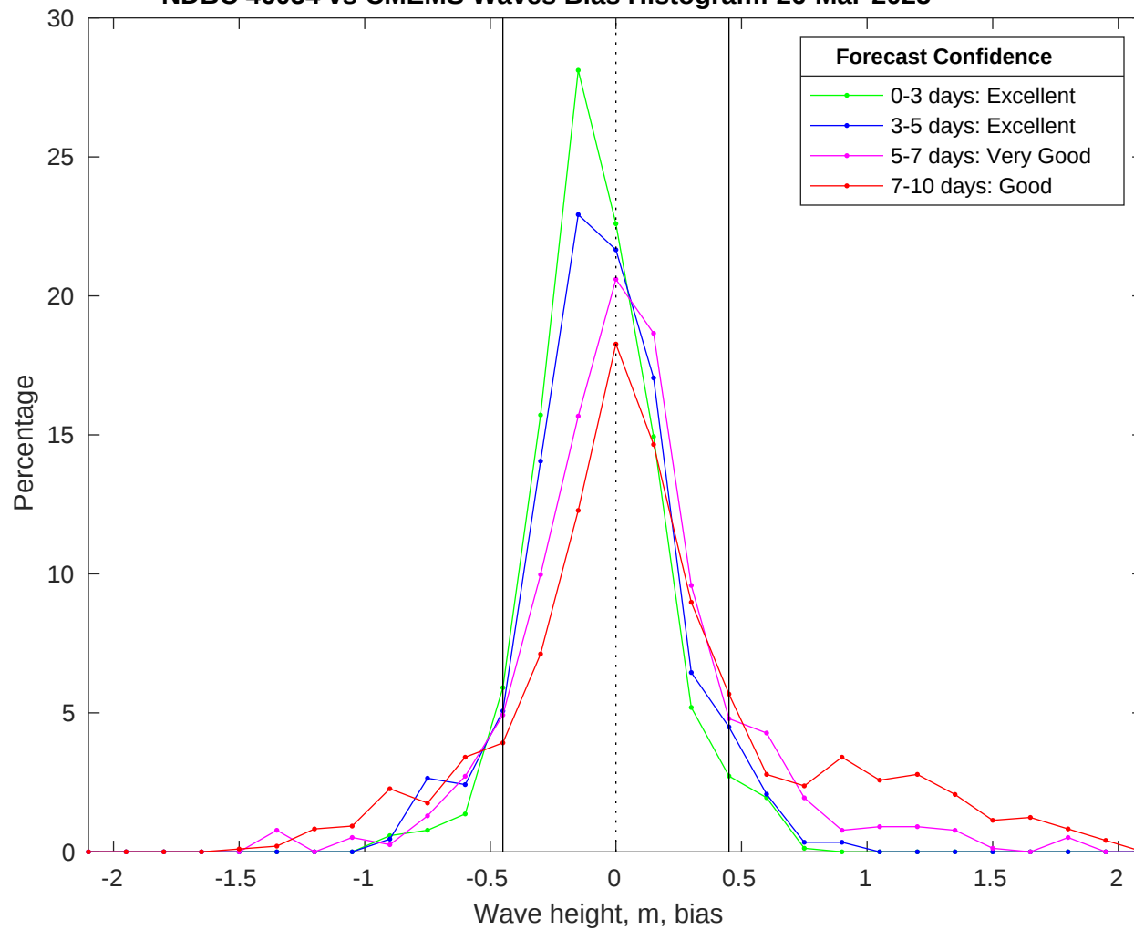
NDBC 46054 vs CMEMS Waves Bias Histogram: 26-Mar-2025
