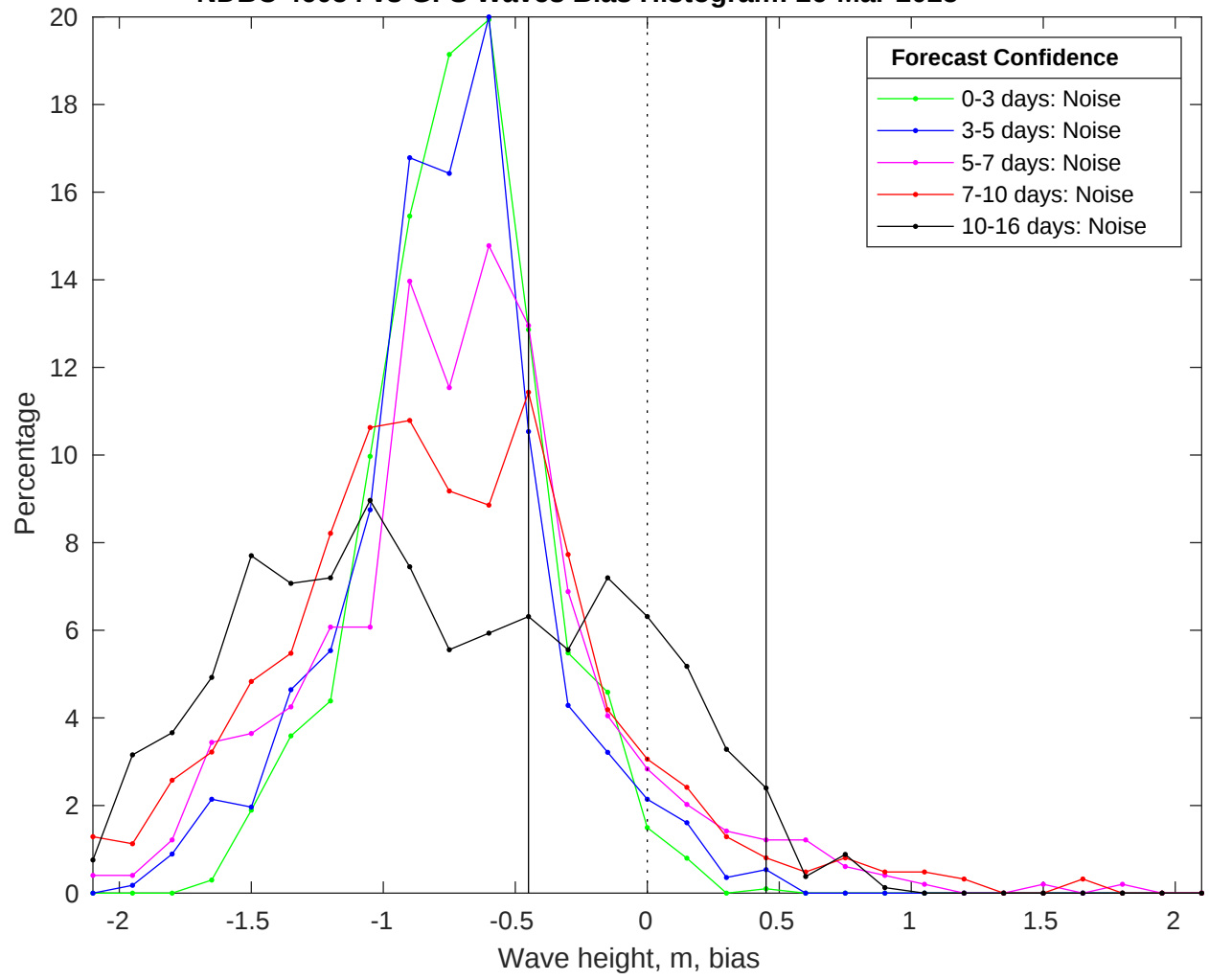
NDBC 46054 vs GFS Waves Bias Histogram: 26-Mar-2025
