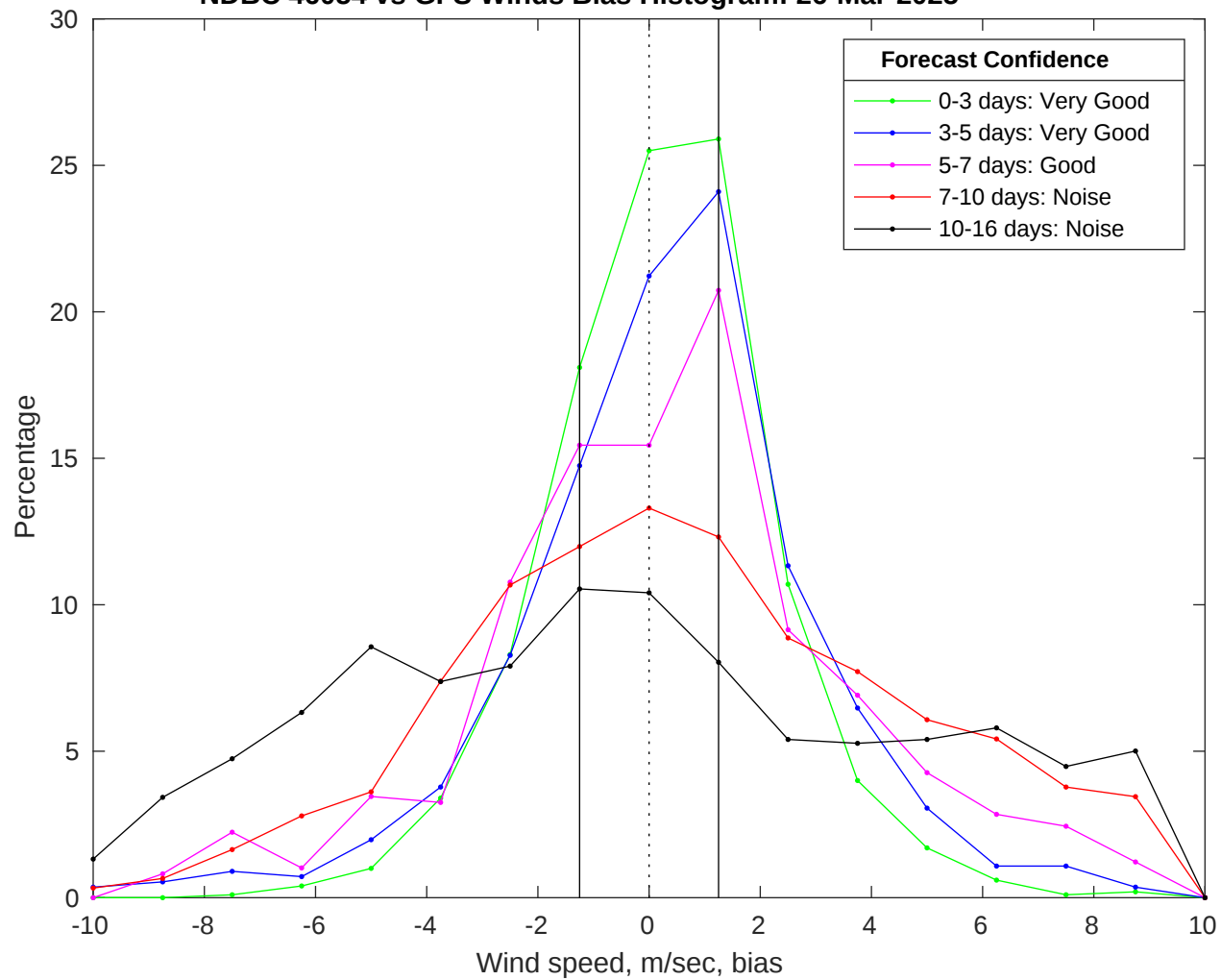
NDBC 46054 vs GFS Winds Bias Histogram: 26-Mar-2025
