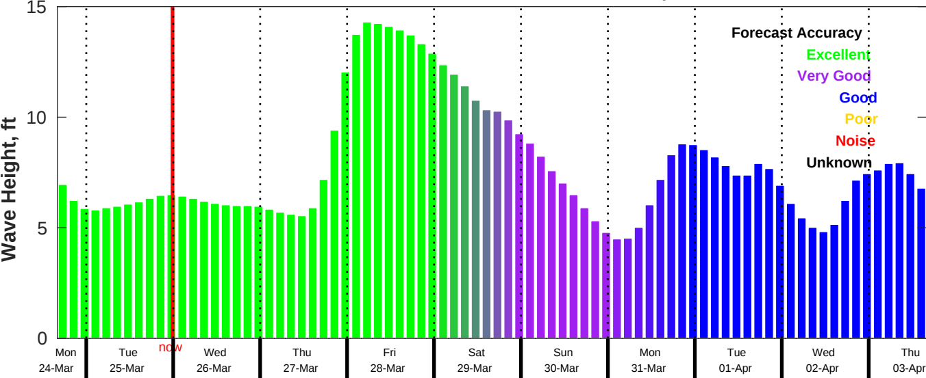
CMEMS Wave Forecast for NDBC 46054 from 24-Mar-2025 16:00:00 to 03-Apr-2025 16:00:00
