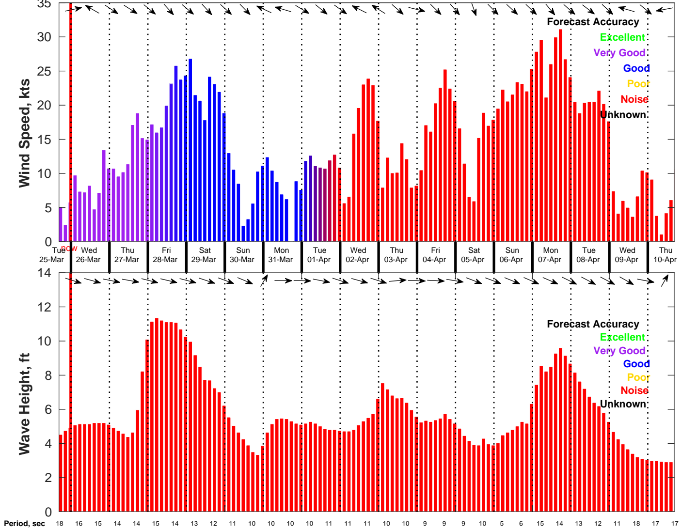
Wind & Wave Forecast for NDBC 46054 from 25-Mar-2025 16:00:00 to 10-Apr-2025 16:00:00
