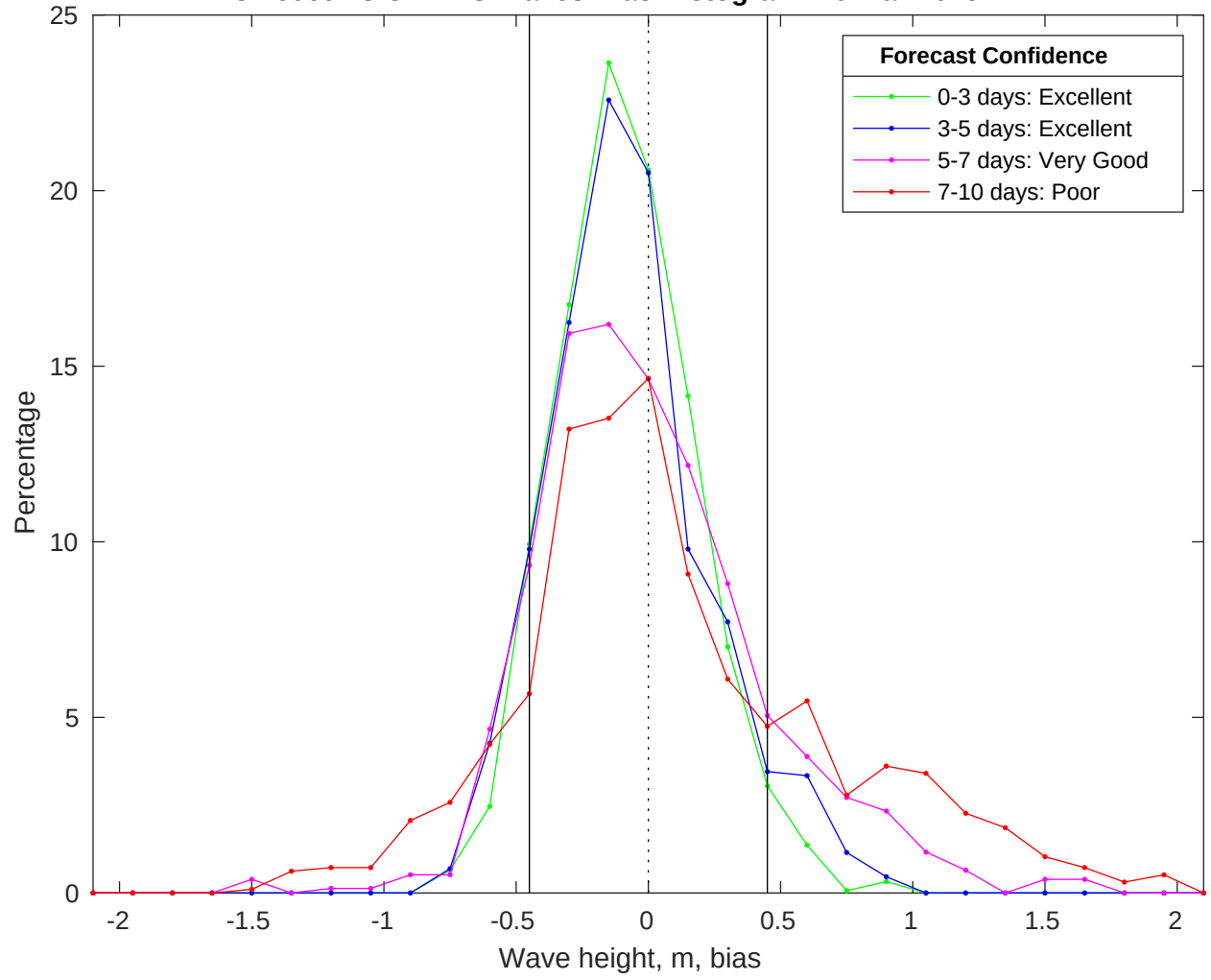
NDBC 46069 vs CMEMS Waves Bias Histogram: 26-Mar-2025
