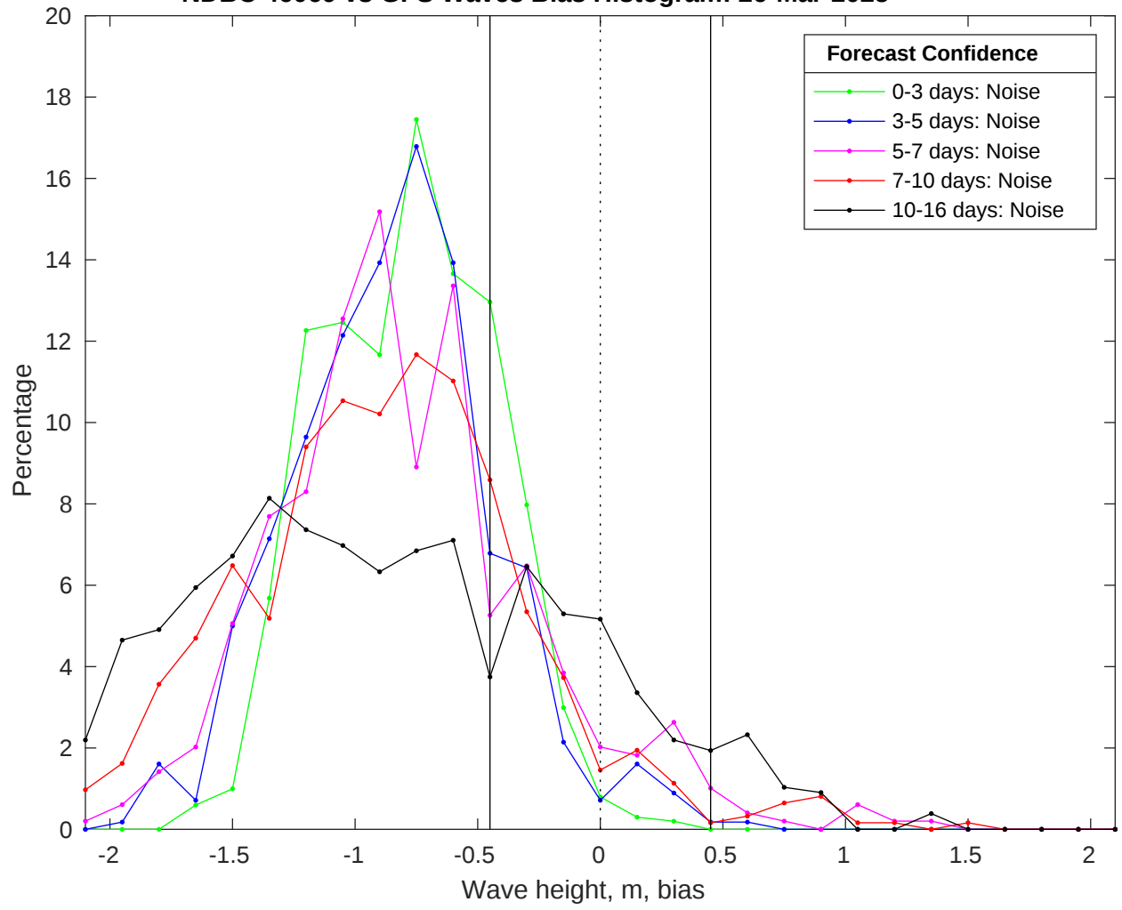
NDBC 46069 vs GFS Waves Bias Histogram: 26-Mar-2025
