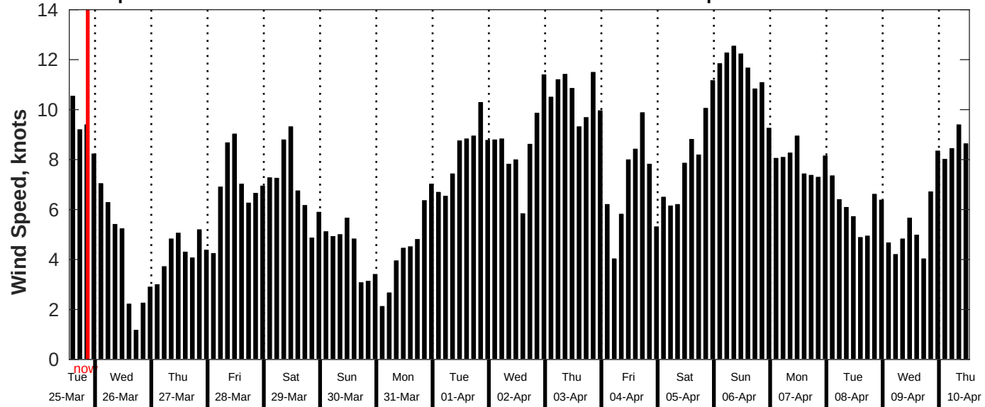
GFS Wind Speed Forecast for NDBC 51209 from 25-Mar-2025 13:00:00 to 10-Apr-2025 13:00:00
