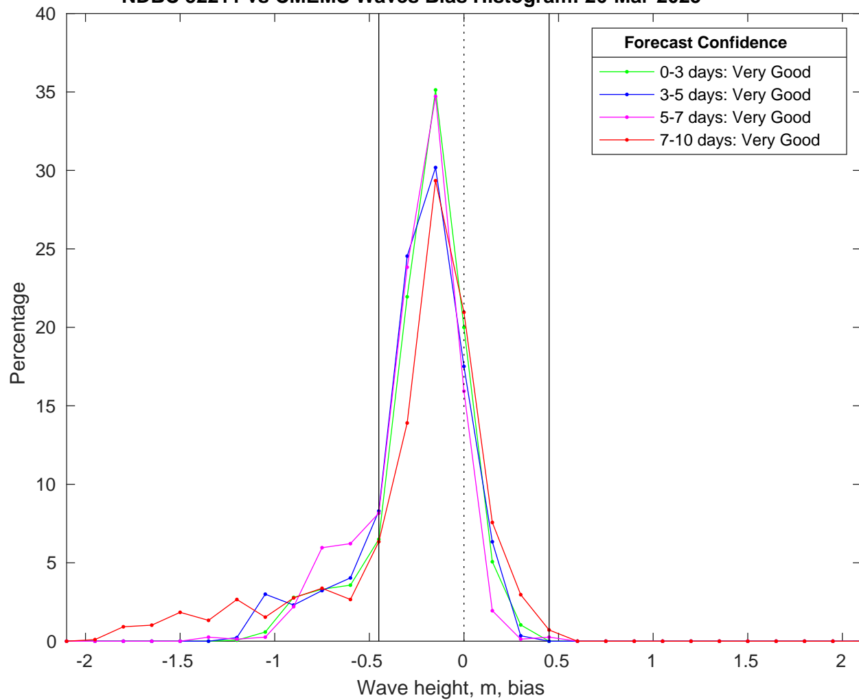
NDBC 52211 vs CMEMS Waves Bias Histogram: 26-Mar-2025
