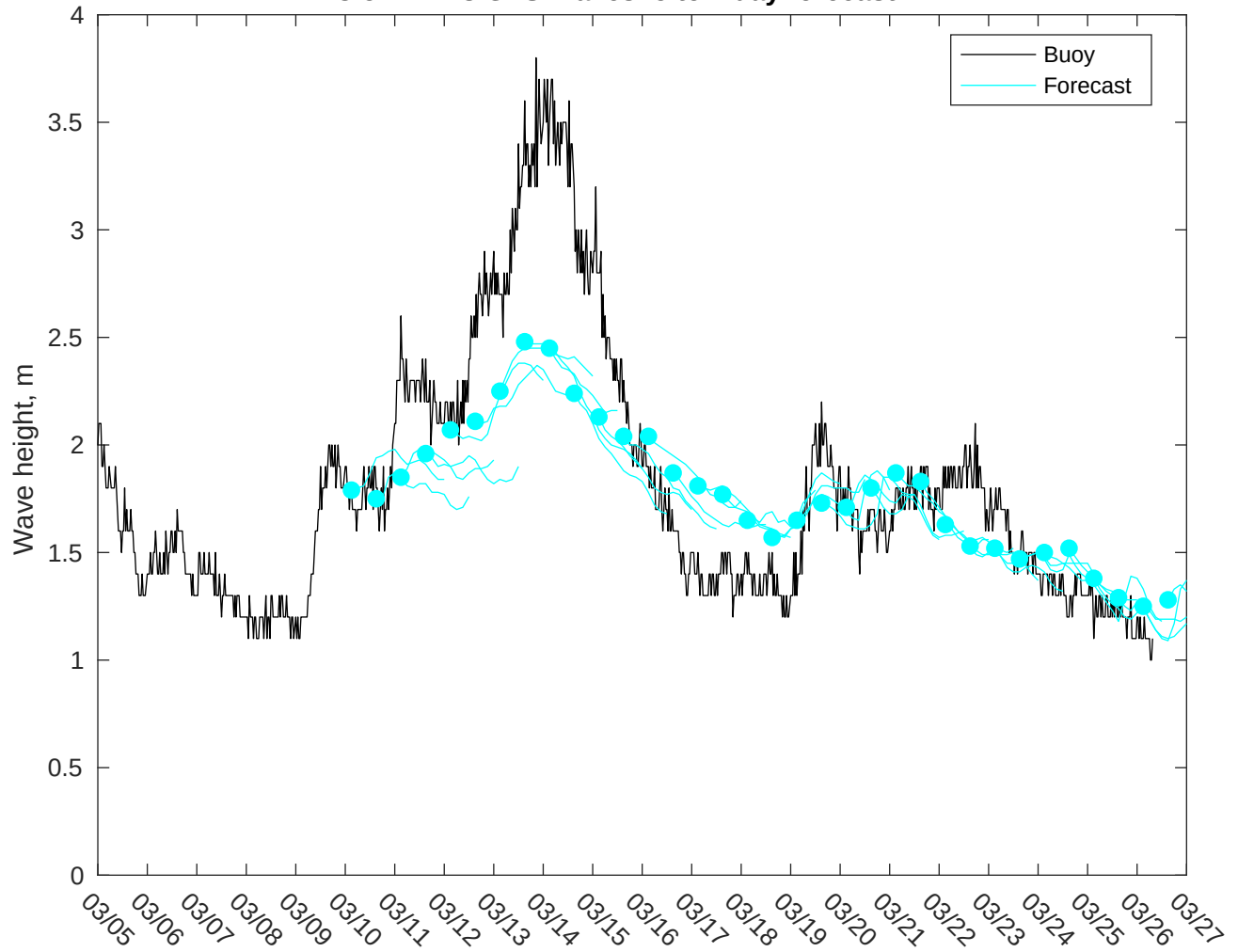
NDBC 52211 vs GFS Waves: 5 to 7 day forecast
