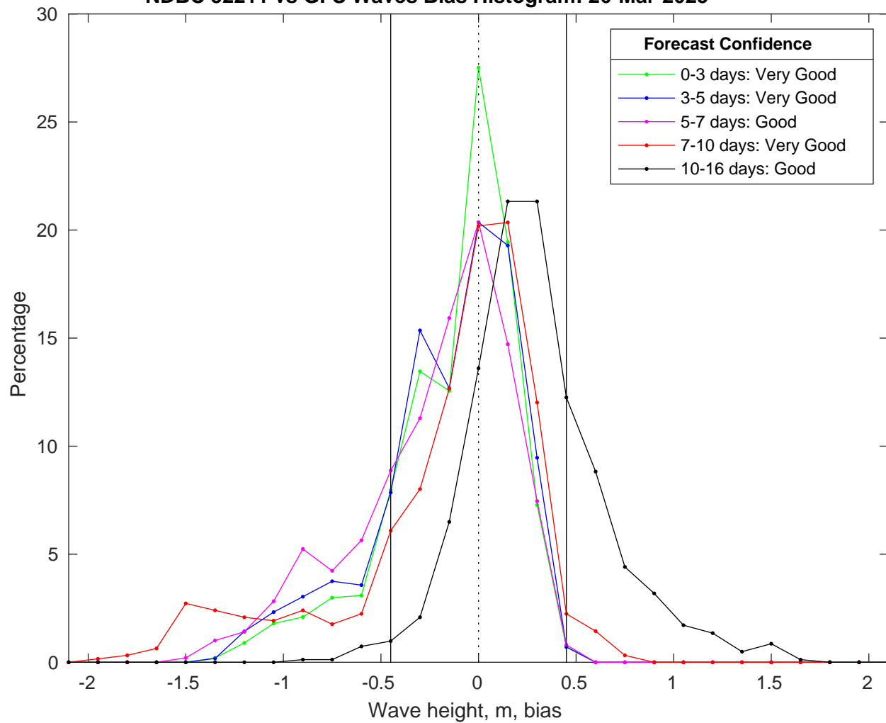
NDBC 52211 vs GFS Waves Bias Histogram: 26-Mar-2025
