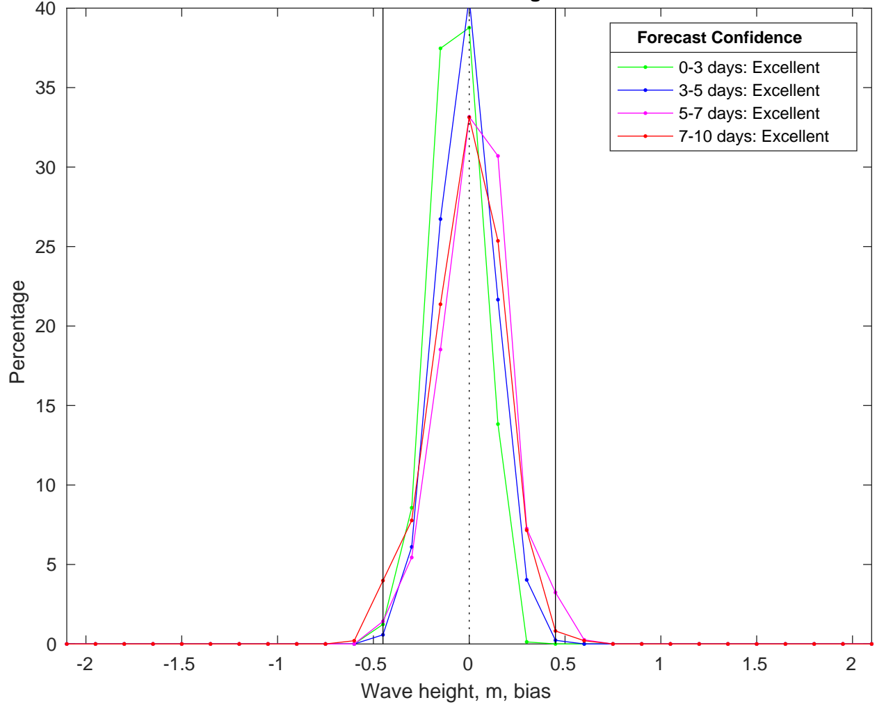
NDBC 52212 vs CMEMS Waves Bias Histogram: 26-Mar-2025
