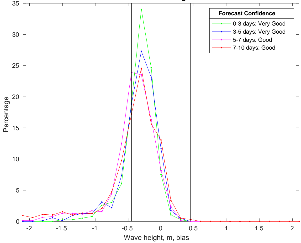
NDBC 52213 vs CMEMS Waves Bias Histogram: 26-Mar-2025
