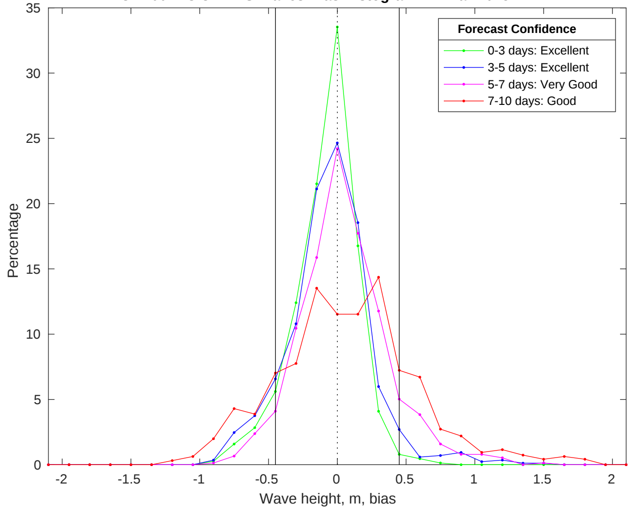
NDBC 41004 vs CMEMS Waves Bias Histogram: 27-Mar-2025
