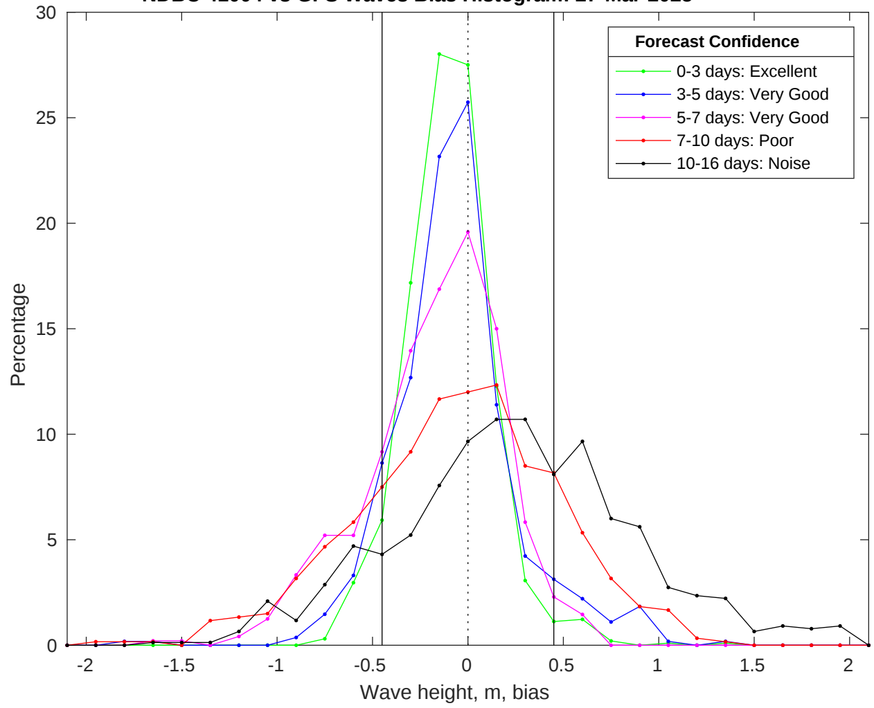
NDBC 41004 vs GFS Waves Bias Histogram: 27-Mar-2025
