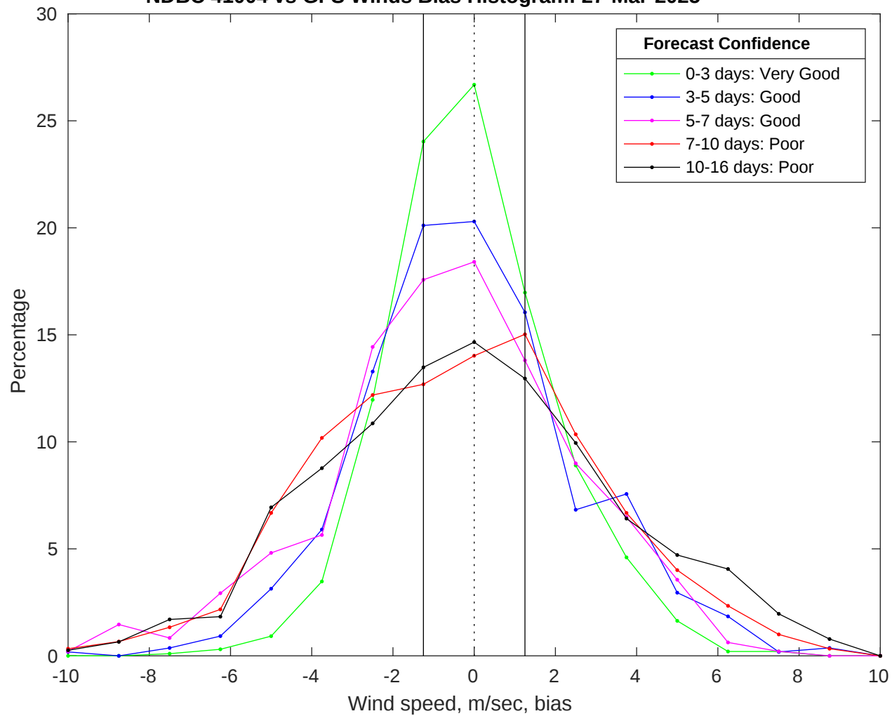
NDBC 41004 vs GFS Winds Bias Histogram: 27-Mar-2025
