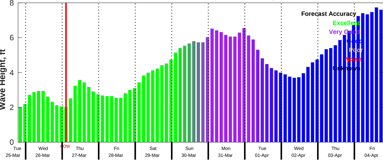
CMEMS Wave Forecast for NDBC 41004 from 25-Mar-2025 19:00:00 to 04-Apr-2025 19:00:00
